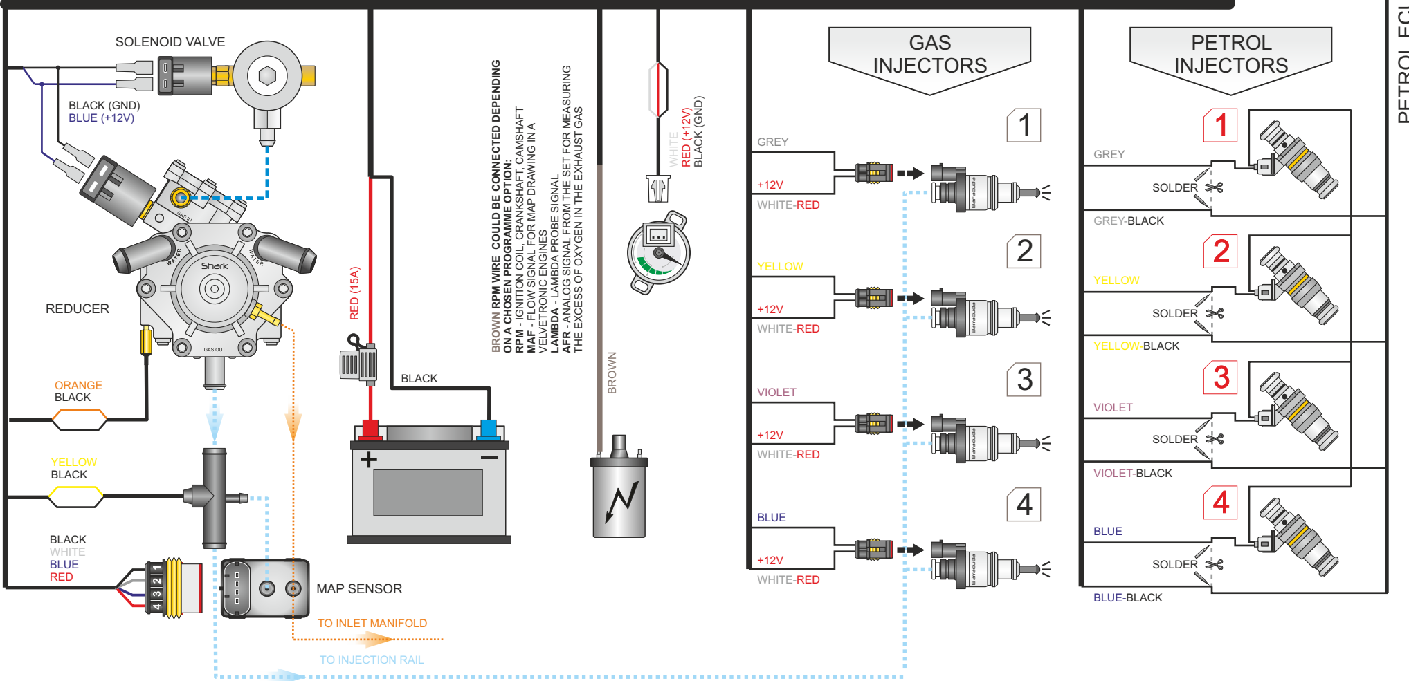
CONNECTION DIAGRAM OF THE LPG/CNG OPTIMA NANO INSTALLATION
